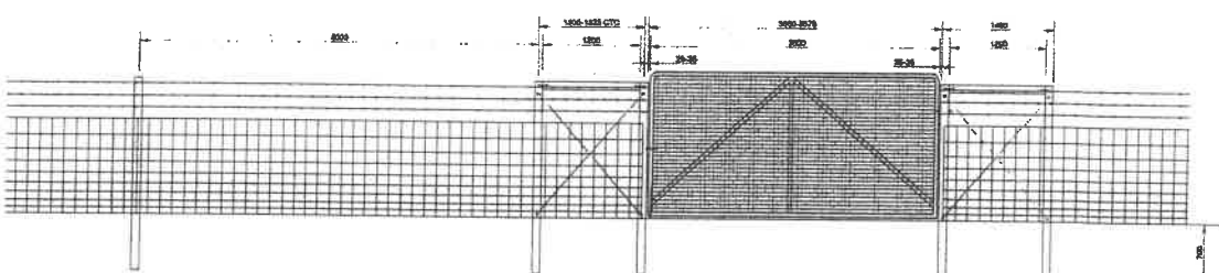
FENCE LINE WITH SINGLE VEHICLE GATE
